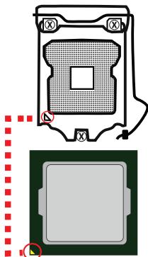
Figure 2-6 CPU installation
