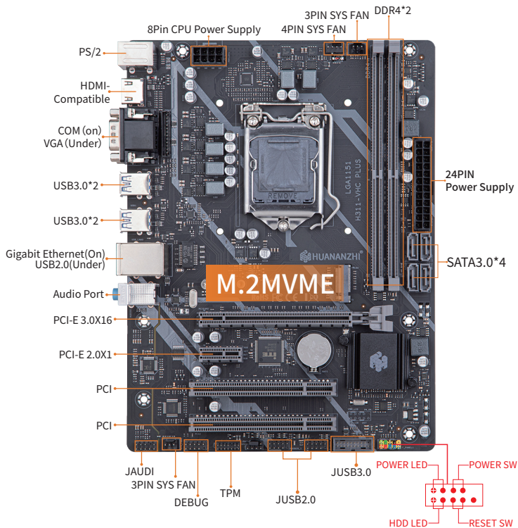
1-1 H311-VHC PLUS motherboard illustration
